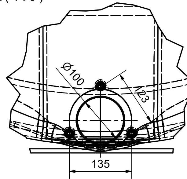
A (1:5)
