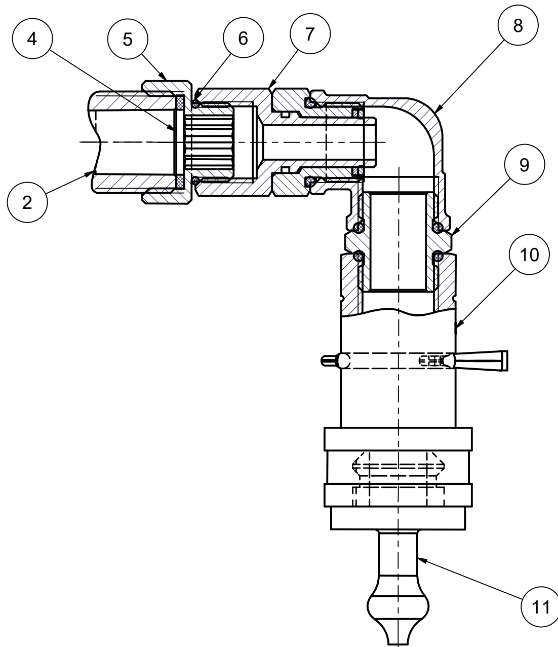
F-F (1:1)
