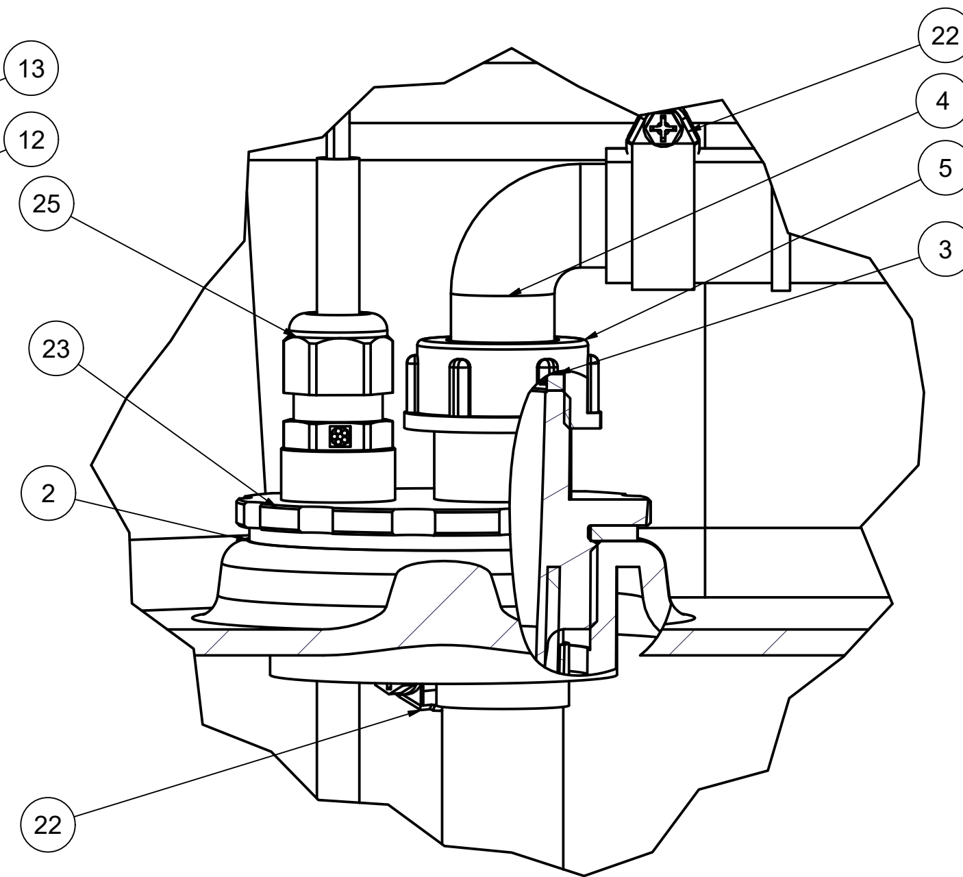
D (1:1)
