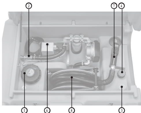
DT-Mobil Easy 980 Premium with CENTRI SP80
