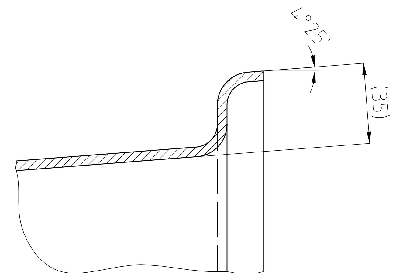
B - B (1:1)
